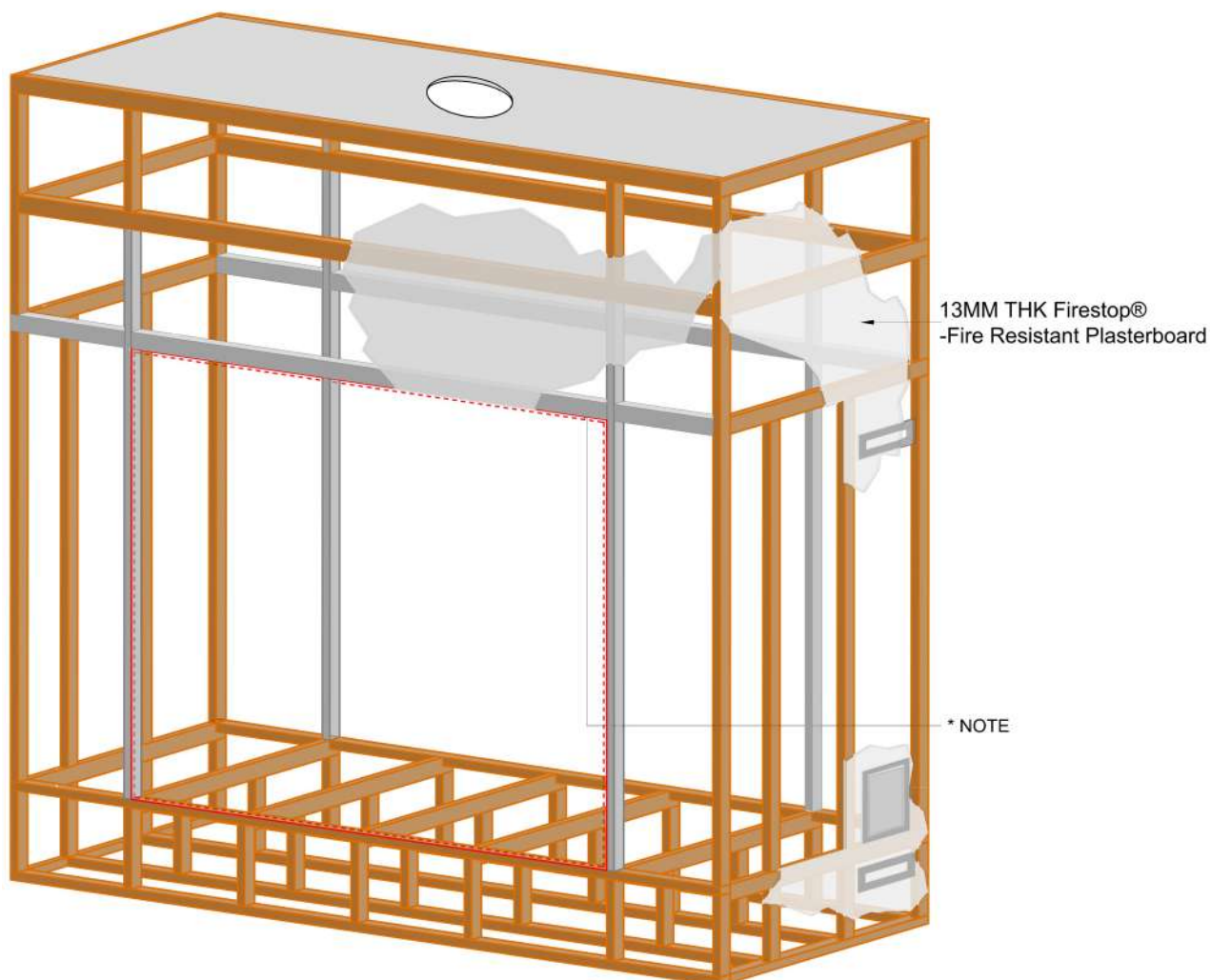
Figure 1.7 (Cladding Material)
