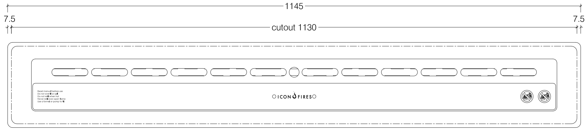
Top View
