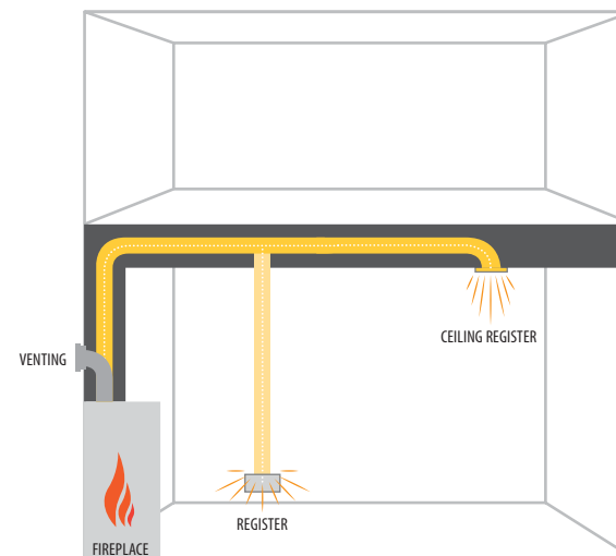
Optional Heat Distribution Kit
